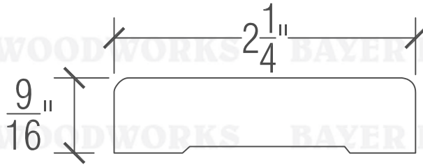
157A CASING
