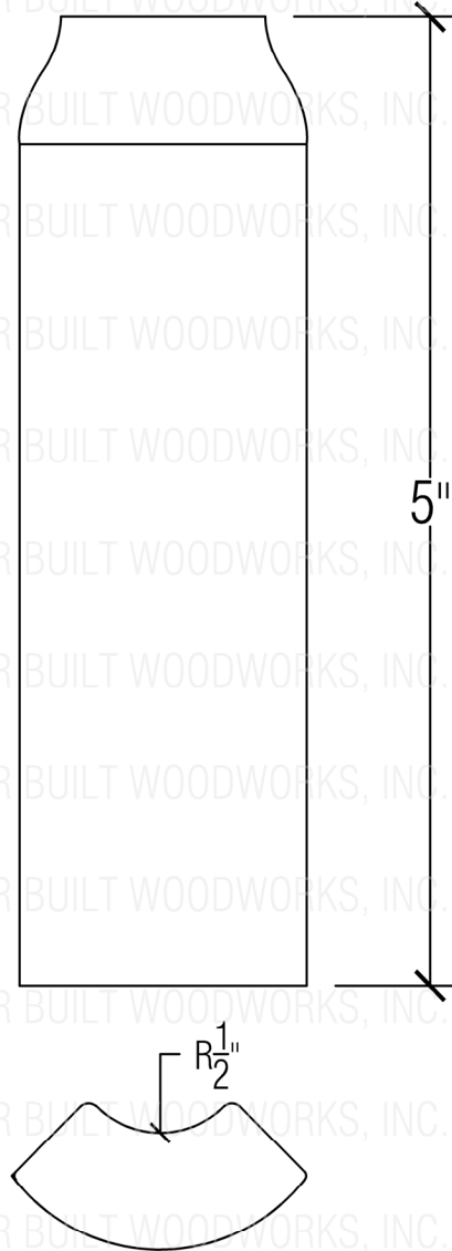
259B Block - \frac{1}{2} " Radius Accepts Up To \frac{1}{2} " Base
