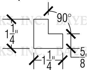
269A Block
