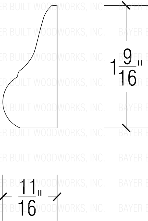
705A PANEL MOULD
