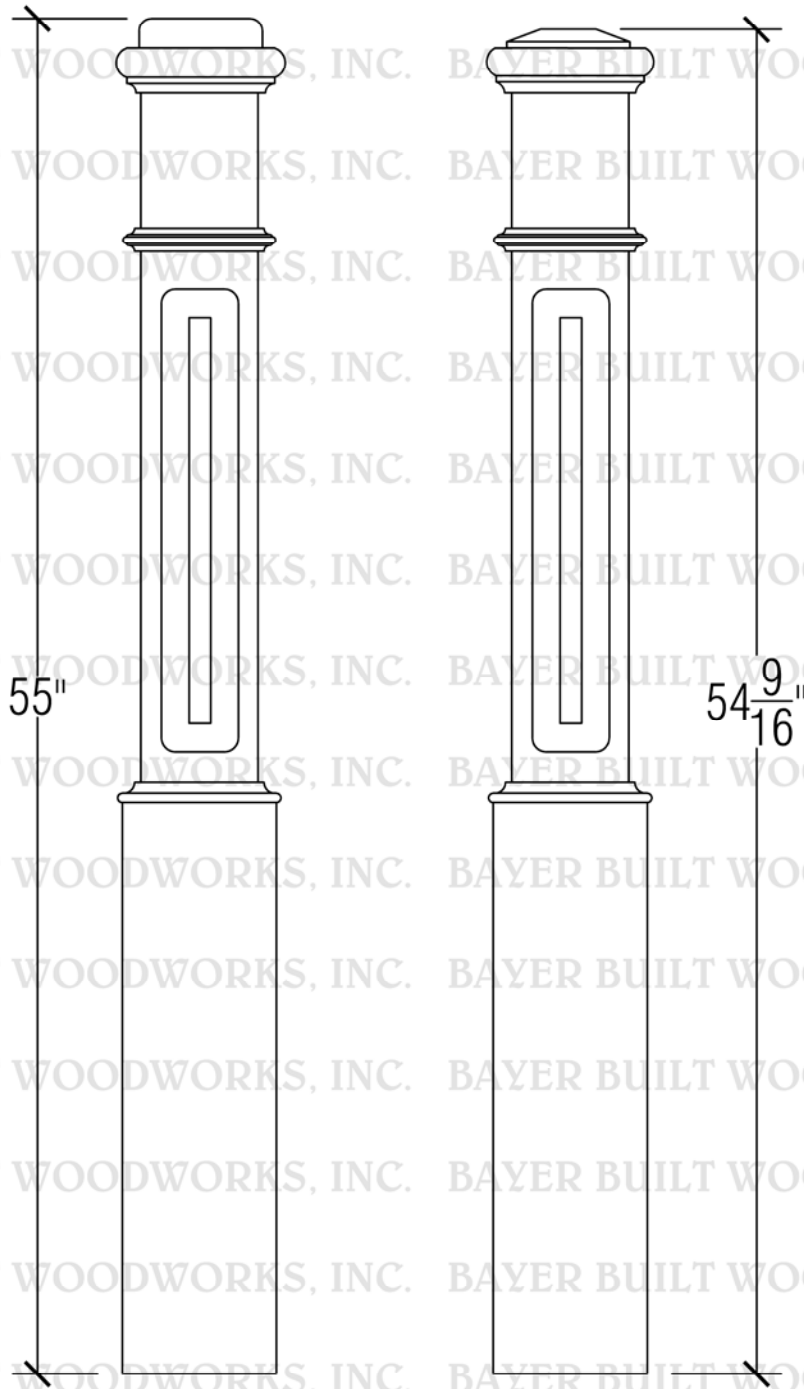
4091-RP BOX NEWEL
