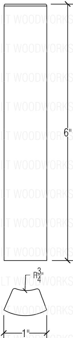
260G Block - \frac{3}{4}" Radius Accepts Up To \frac{1}{2}" Base
