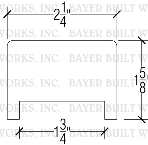
6770P1 RAIL
