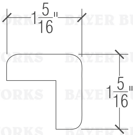
653A OUTSIDE CORNER
