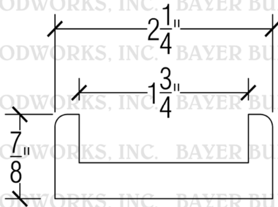
6002 SHOE RAIL
