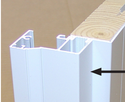
1/2" Reveal - brickmould is 1/2" from jamb face.
